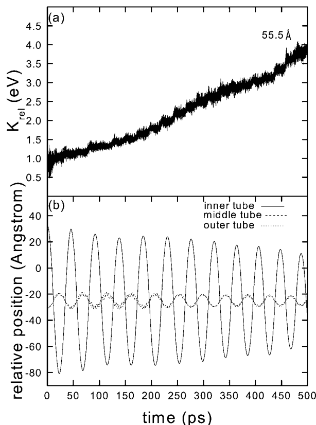
Figure 8. (a) Calculated K_{rel}(t) for a TWNT oscillator (70/70/55 Å) and s = 55.5 Å. (b) Centre-of-mass displacements of three nanotubes along the translational direction.
