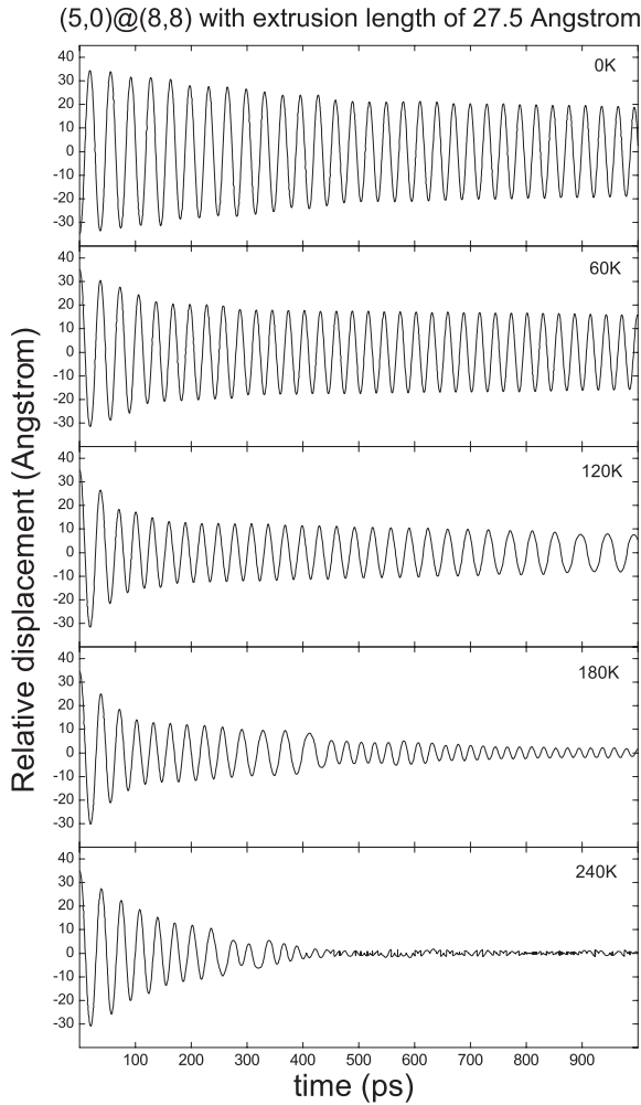
Figure 11. Relative displacement as a function of time for s = 27.5 \text{ \AA} and five different initial temperatures: 0, 60, 120, 180, 240 K.
