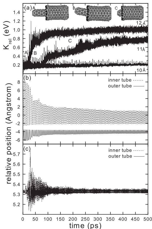
Figure 3. (a) Calculated K_{\text{rel}}(t) of capped oscillator for three values of s = 10, 11 and 12 \text{ \AA} . Configurational graphs are drawn for (A) before the onset of the rocking motion, (B) during the rocking motion, and (C) after the rocking motion. In all cases except for s = 10 \text{ \AA} , portions of translational energies are transferred into K_{\text{rel}}(t) within 100 ps from the start of the simulation. (b) The centre-of-mass displacements of two nanotubes along translational direction for s = 12 \text{ \AA} . (c) The centre-of-mass displacements of two nanotubes perpendicular to translational direction for s = 12 \text{ \AA} .
