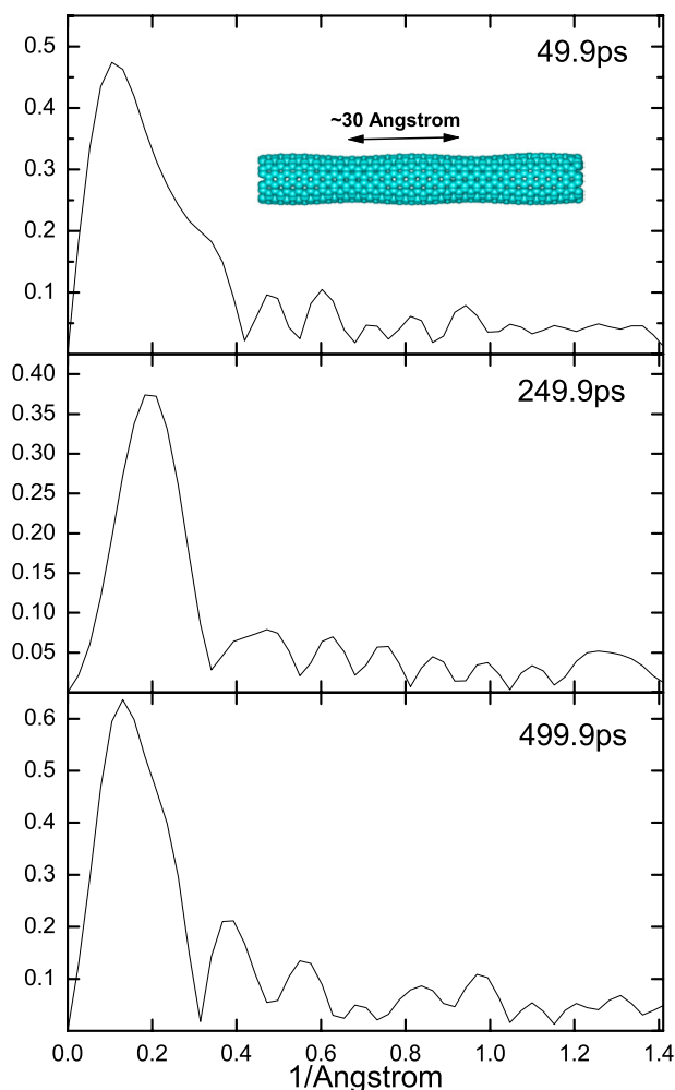
Figure 5. Fourier transforms of carbon atom displacements in a direction perpendicular to the translational oscillation of the long-tube combination (70/55 Å) for an initial extrusion length s = 27.5 Å. Three snapshots are selected: (a) t = 49.9 ps, (b) t = 249.9 ps, and (c) t = 499.9 ps.
