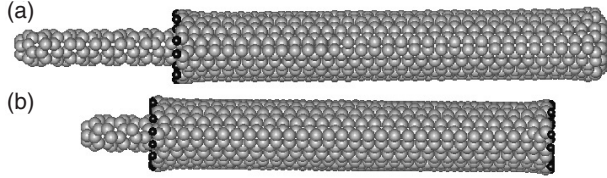
Figure 1. Illustrative examples of (a) one-end capped and (b) uncapped DWNT oscillators.
