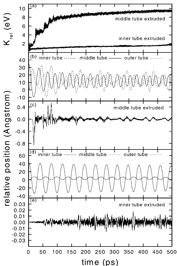
Figure 9. (a) Calculated K_{rel}(t) of a TWNT oscillator (70/70/55 Å) with the inner or middle tube extruded initially by a length s = 35 Å. Up to 500 ps of oscillational motion have been simulated. (b) Centre-of-mass displacements of three nanotubes (solid, middle tube; dashed, inner tube; dotted, outer tube) along the translational direction when initially the middle tube is extruded. (c) Centre-of-mass displacements of inner tube perpendicular to the translational direction when initially the middle tube is extruded. (d) Centre-of-mass displacements of three nanotubes along the translational direction (solid, inner tube; dashed, middle tube; dotted, outer tube) when initially the inner tube is extruded. (e) Centre-of-mass displacements of the inner tube perpendicular to the translational direction when initially the inner tube is extruded.
