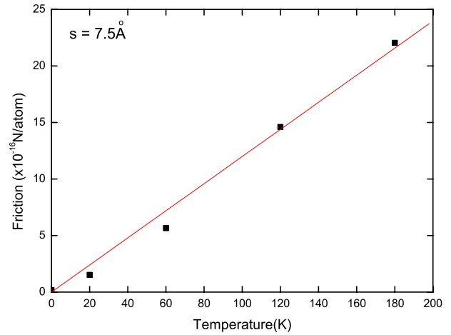
Figure 12. Frictional force per atom (in 10^{-16} N/atom) as a function of pre-simulation heating temperature (in kelvin) for an initial extrusion length s = 7.5 \text{ \AA} . The temperature dependence can be fitted with 0.12T (in 10^{-16} N/atom) as shown by the solid line.
