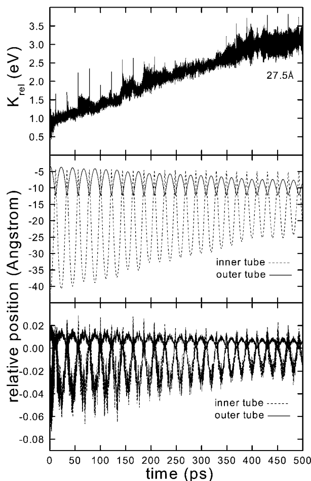
Figure 7. (a) Calculated K_{\text{rel}}(t) of the capped long-tube combination ( 70/55 \text{ \AA} ) for an extrusion length s = 27.5 \text{ \AA} . Up to 500 ps of oscillation is simulated. (b) Centre-of-mass displacements of two nanotubes along the translational direction. (c) Centre-of-mass displacements of two nanotubes perpendicular to the translational direction.
