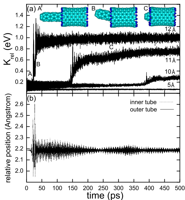
Figure 2. (a) Calculated K_{\text{rel}}(t) of uncapped short-tube oscillators for four values of s = 5, 10, 11, and 12 \text{ \AA} . Configurational graphs are drawn for (A) before the onset of the rocking motion, (B) during the rocking motion, and (C) after the rocking motion. In all cases except for s = 5 \text{ \AA} , portions of translational energies are transferred into K_{\text{rel}}(t) within 400 ps from the start of the simulation. (b) The centre-of-mass displacements of two nanotubes perpendicular to the translational direction for s = 12 \text{ \AA} .
