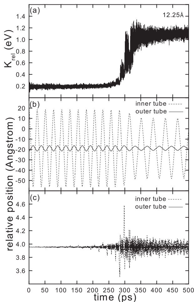
Figure 4. (a) Calculated K_{\text{rel}}(t) of mixed-tube combination ( 70/14.5 \text{ \AA} ) with s = 12.25 \text{ \AA} . (b) The centre-of-mass displacement of two nanotubes along the translational (axial) direction. (c) The centre-of-mass displacement of two nanotubes in a radial direction.
