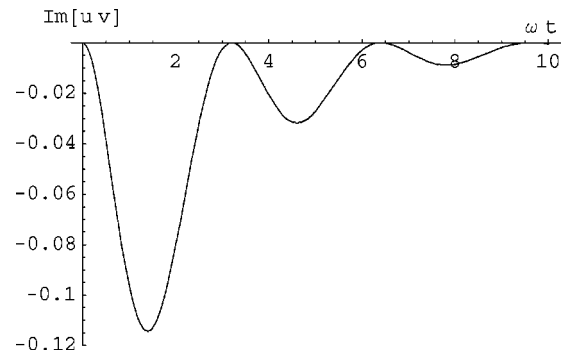
FIG. 3. \text{Im}(uv) for an underdamped case: \gamma/\omega = 0.2 . The initial state is a coherent state.
