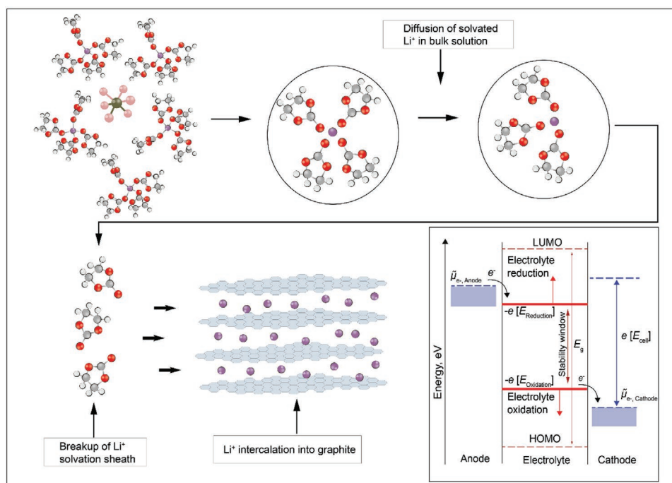
Figure 4. (Top) Example of interfacial electrolyte structure as solvated Li (in this example Li is coordinated to EC in the presence of \text{PF}_6^- anion) diffuses and intercalates on the anode surface. The multi-component nature of the electrolyte highlights the complexity of the electrode/electrolyte interface in terms of electrochemical stability, structure, and dynamics. (Bottom) Electrochemical stability window of battery electrolytes; inspired by Peljo and Girault. [92]
